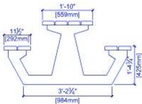
Side Elevation
