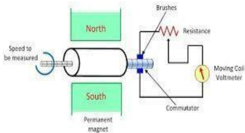
DC Tachometer Generator
