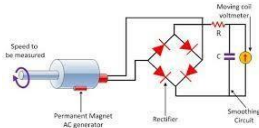
A.C Tachometer Generator
