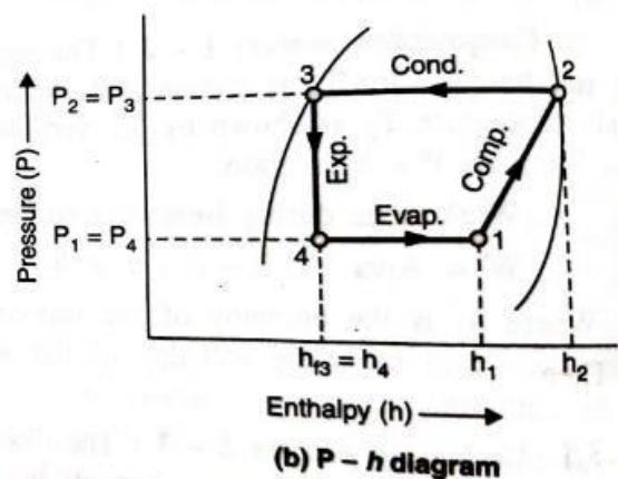
Fig. 2.5 Vapour compression cycle for wet compression
