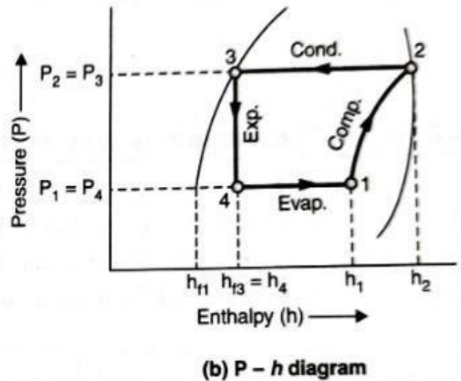
Fig. 2.4 Vapour compression cycle for dry compression
