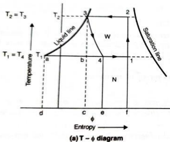
Fig. 2.5 Vapour compression cycle for wet compression
