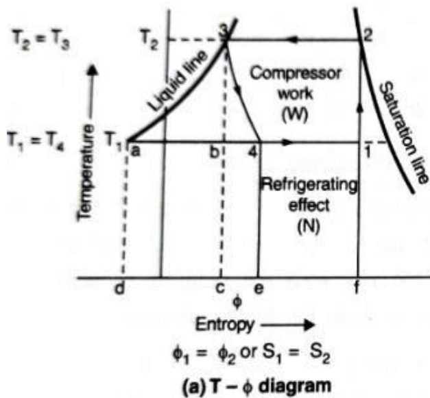
Fig. 2.4 Vapour compression cycle for dry compression
