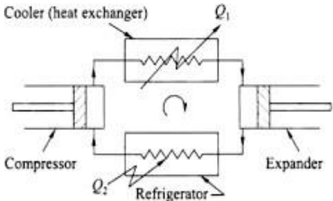
Fig.1.6 Air Expansion Refrigeration
