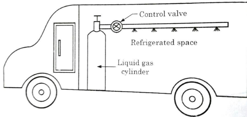
Fig.1.4 Liquid Gas Refrigeration
