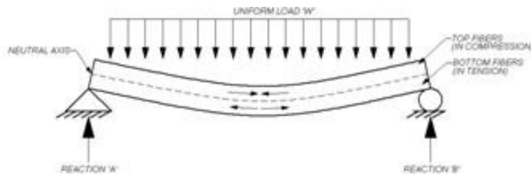
Figure 1-Beam diagram
